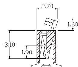
SECT X-X
